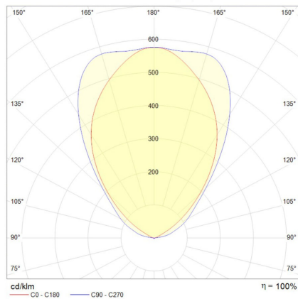
Verne Midi Wall Washer 70° x 55° (Asym.)
