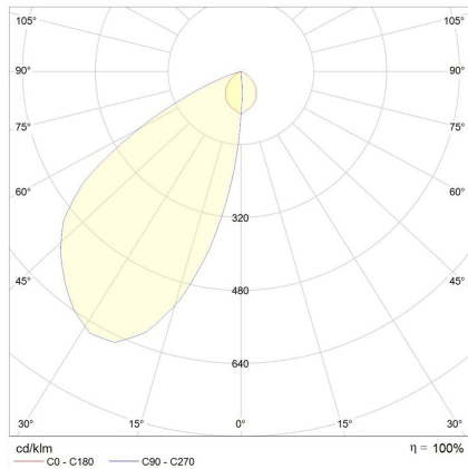
Toulouse Rectangle Recessed 60°
