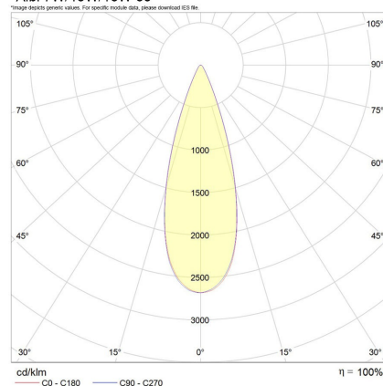
*Albi 7W/13W/18W 30°
