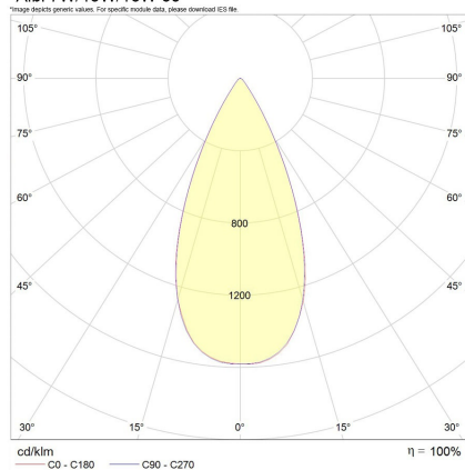
*Albi 7W/13W/18W 50°
