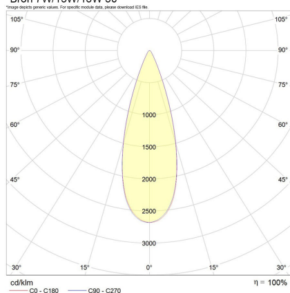
*Bron 7W/13W/18W 30°
