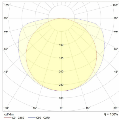
Linea COB LED 10W 140°
