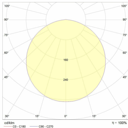
Neonflex Side Bendable 120°
