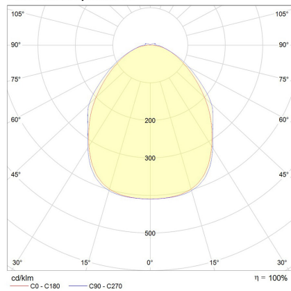
Pesaro Maxi Adjustable 90°
