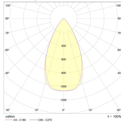
Pesaro Maxi Adjustable 60°
