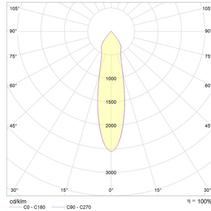
Benson Adjustable 25°
