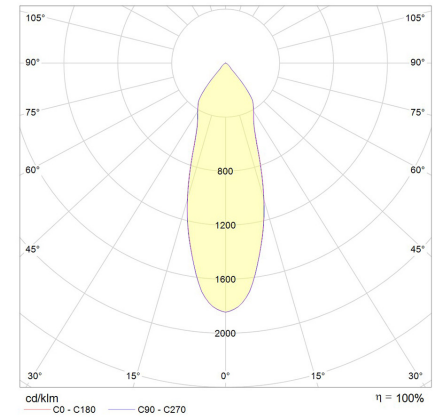
Benson Adjustable 35°
