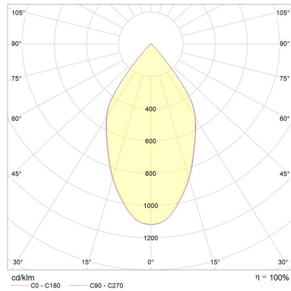
Benson Adjustable 60°
